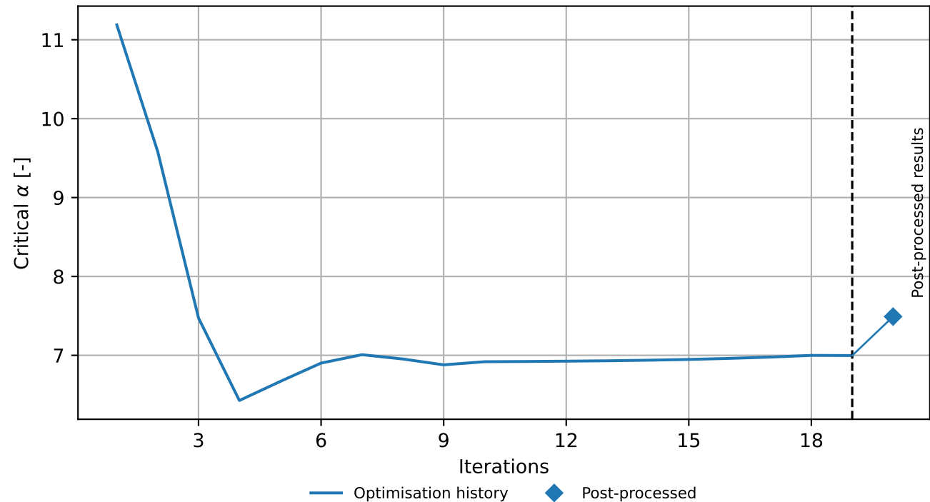
SLP Critical alpha convergence
